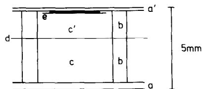
Fig. 1. Anaerobic microscope slide chamber. A diagrammatic cross section is shown. A sample is placed under a circular coverslip (e) on a larger rectangular coverslip ( a' ). A sandwich is assembled using 2 silicone rubber rings (b) and a Teflon membrane (d) to create the upper ( c' ) and lower (c) compartments. The whole assembly sits on a microscope slide in a metal chamber with viewing ports. The lower compartment was filled with sodium dithionite in dilute NaOH by injecting in through the silicone rubber ring (b).
